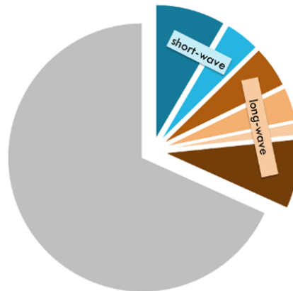
Figure 2 – Execution time of WRF model subdivided in terms of modules and kernels. Only the radiation driver has been highlighted and further split into short-wave and long-wave computations
